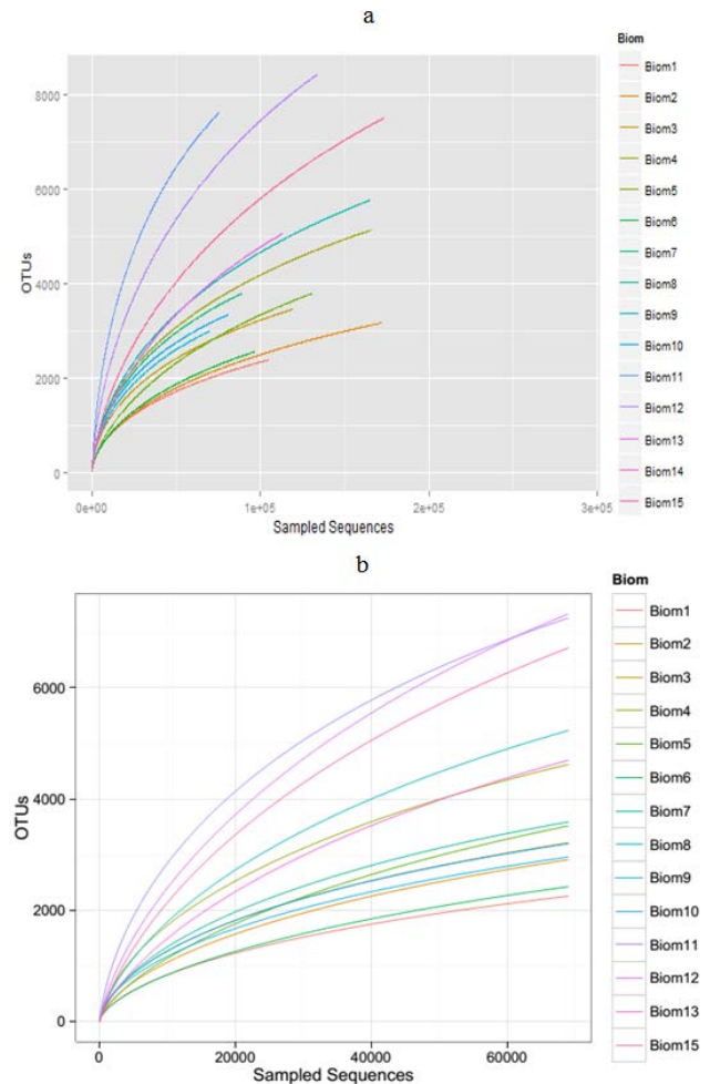
Figure 2. Rarefaction curves of v4 region of 16S rRNA gene sequences from 15 samples. Figure 2a show rarefaction curves as per sequences generated from each sample and Figure 2b is a rarefaction curve after subsampling of 69,000 sequences from each sample
