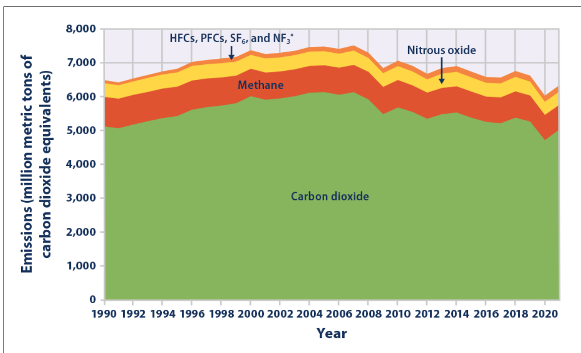
Figure 3: US Greenhouse Gas Emissions by Gas, 1990–2021
